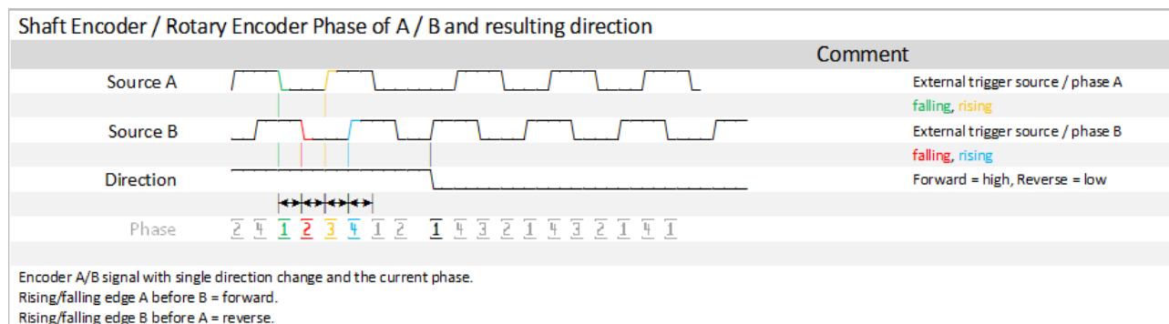
Figure 7.1. Shaft Encoder, A &amp; B phase, direction
